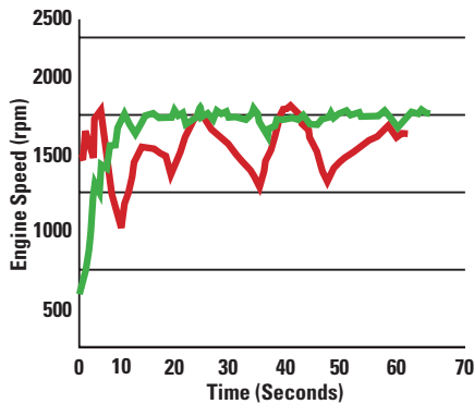
■ With Automatic Retarder Control (average speed, 1950 rpm) ■ With Manual Retarder Control (average speed, 1730 rpm)
